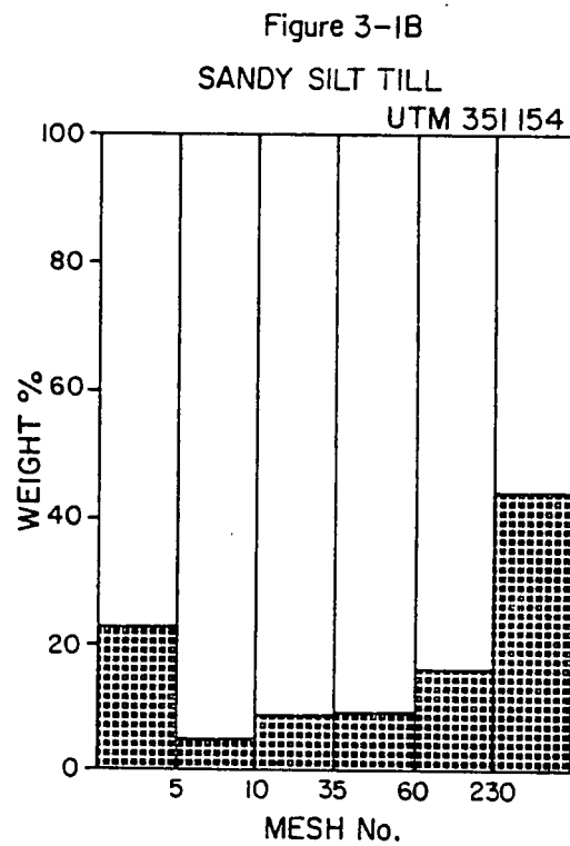
Figure 3-1 REPRESENTATIVE GRAIN SIZE DISTRIBUTIONS
