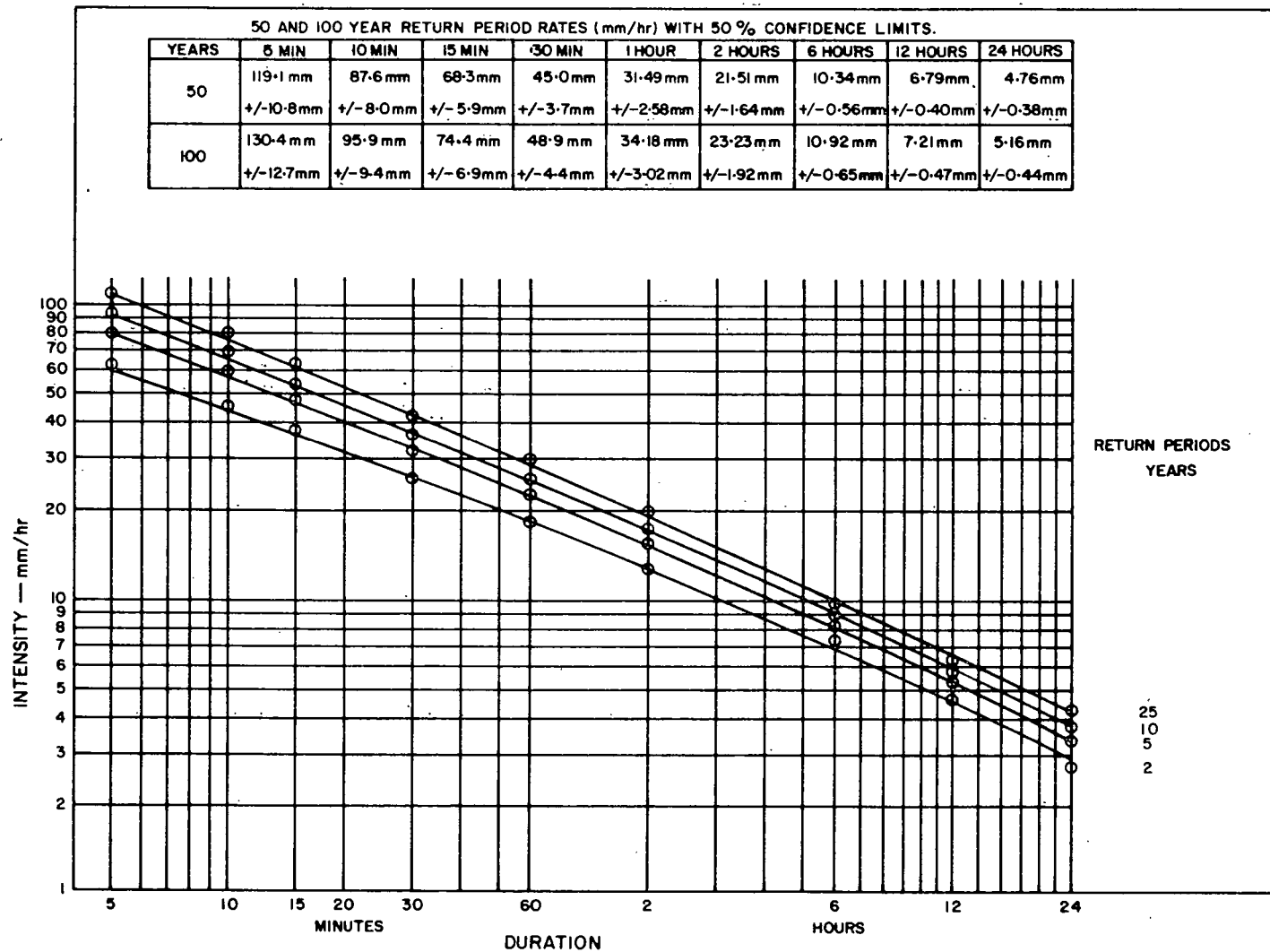
Figure 4-2 SHORT DURATION RAINFALL INTENSITY-DURATION FREQUENCY DATA FOR SYDNEY BASED ON RECORDING RAIN GAUGE DATA FOR THE PERIOD -1961-1979, 18 YEARS
